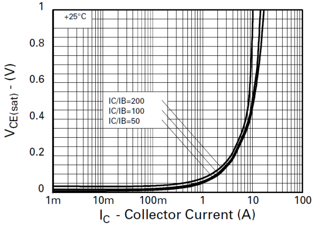
Fig.5 V_{CE(sat)} \text{ v } I_C
