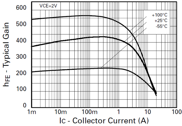
Fig.7 h_{FE} \text{ v } I_C
