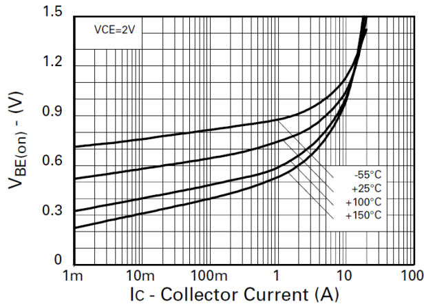
Fig.9 V_{BE(on)} \text{ v } I_C
