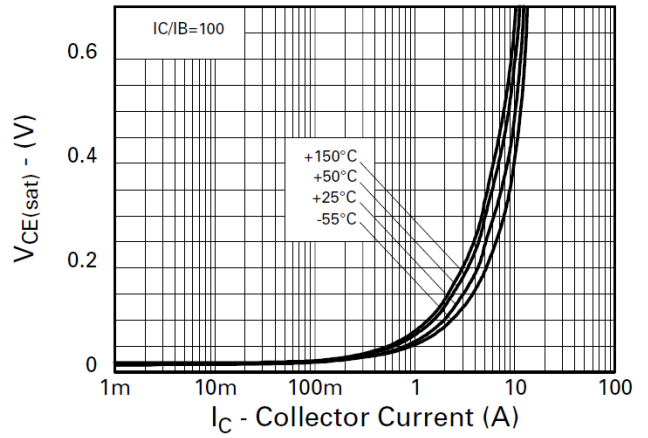
Fig.6 V_{CE(sat)} \text{ v } I_C
