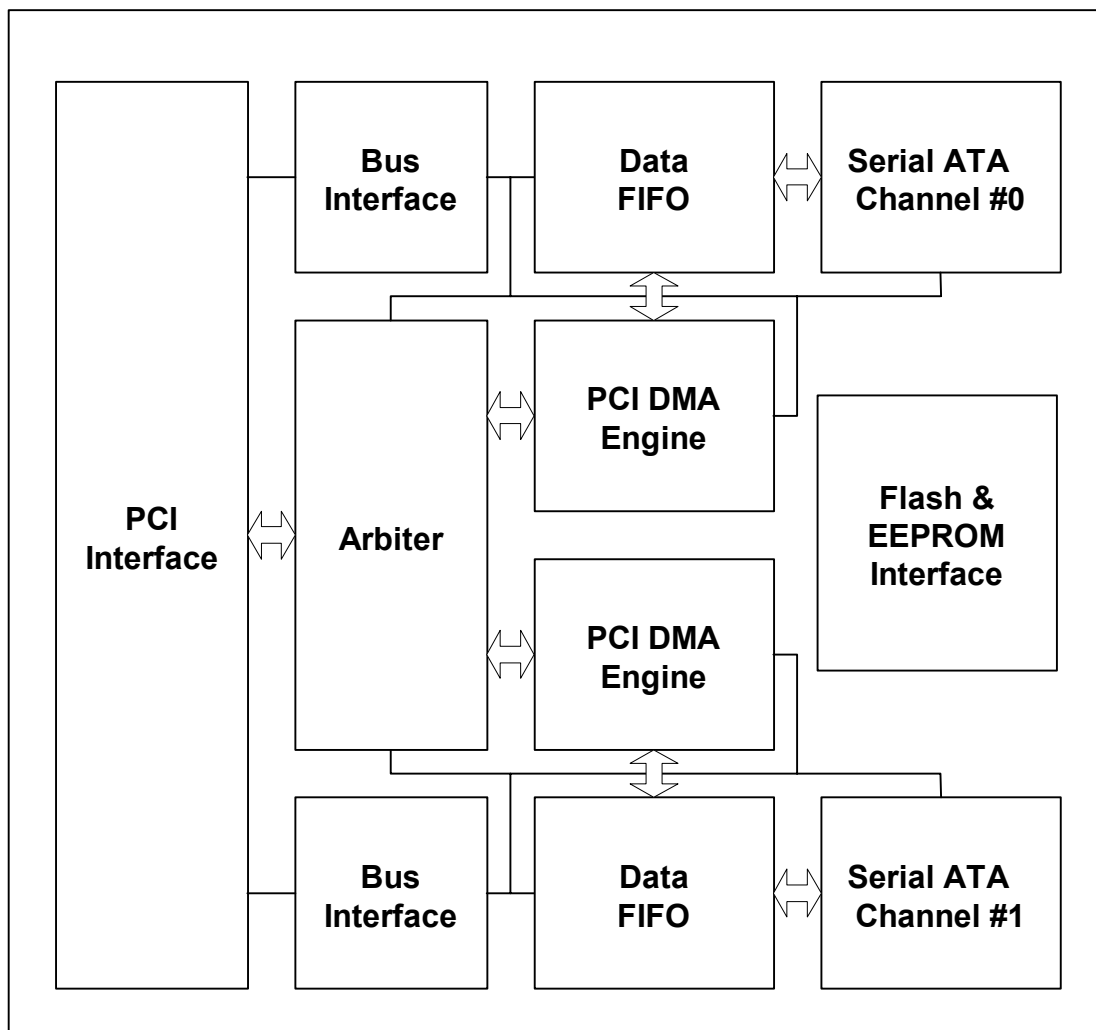
Figure 4-1: SiI3112A Block Diagram
